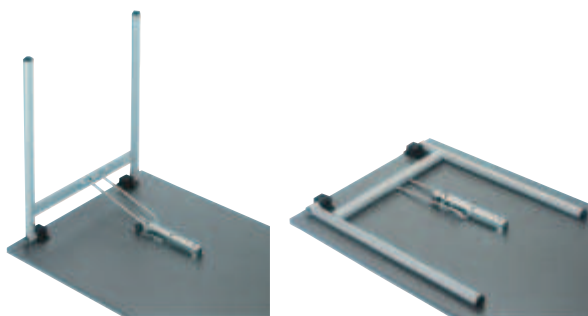
Offset installation H-frame
