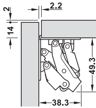
Flap closed
